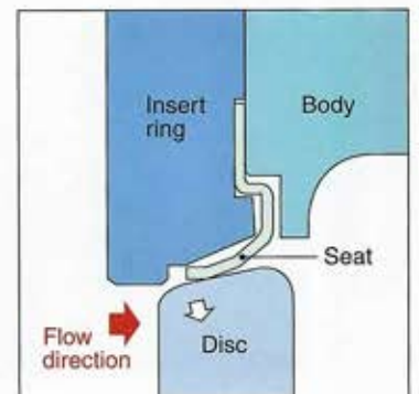
Sealing structure
